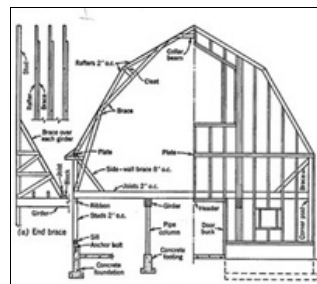
Shawver Truss
